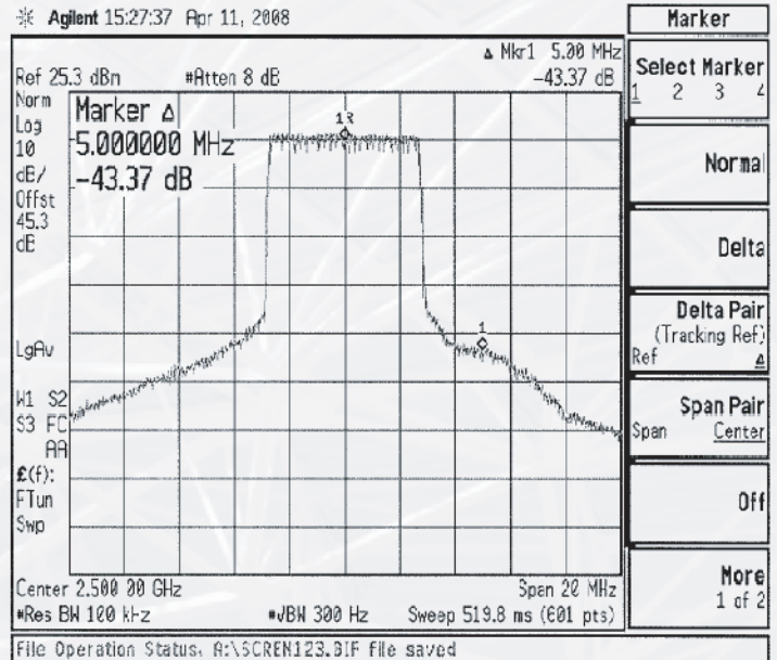
Spectral Regrowth at 2.50GHz
