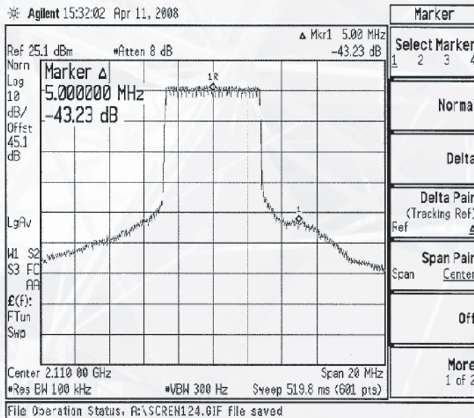
Spectral Regrowth at 2.11GHz
